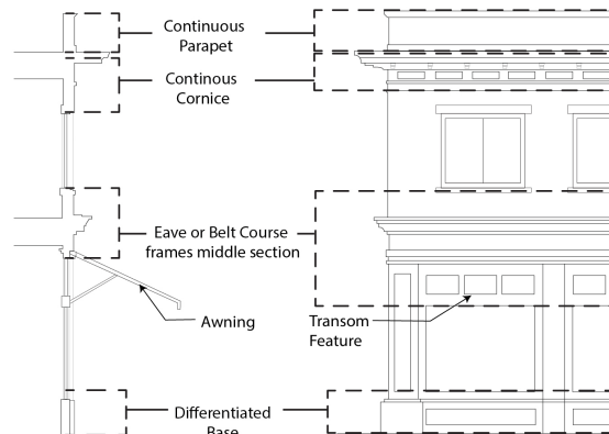
Figure 17.17.040.B: Building Façade Visible from Public Street
