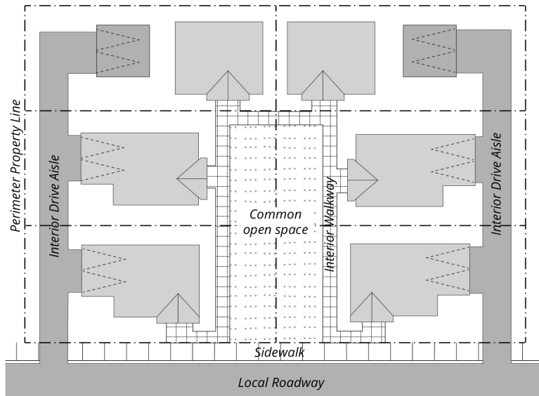
Figure 17.16.040.G: Cottage Court with Perimeter Drive Aisle and Detached or Attached Garages (Example Configuration)
