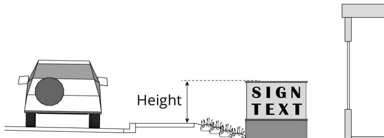
Figure 17.27.060.G: Freestanding Sign Height, Lower Than Adjacent Grade
