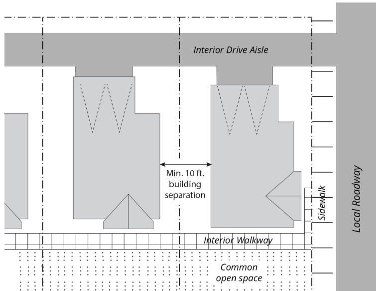
Figure 17.16.040.I: Small Lot Building Separation for Detached Units
