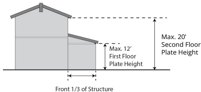
Figure 17.16.040.B: First and Second Story Plate Height
