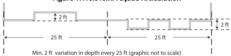
Figure 17.16.040.K: Façade Articulation
