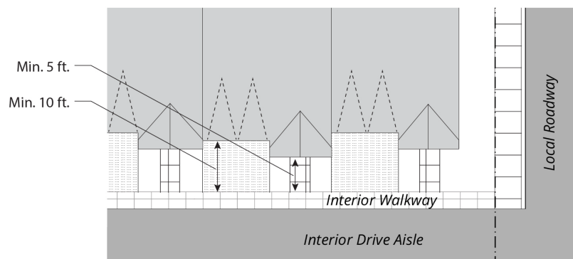
Figure 17.16.040.C: Distance to Interior Drive Aisle or Walkway
