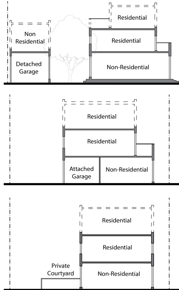
Figure 17.22.140.A: Live/Work Configurations
