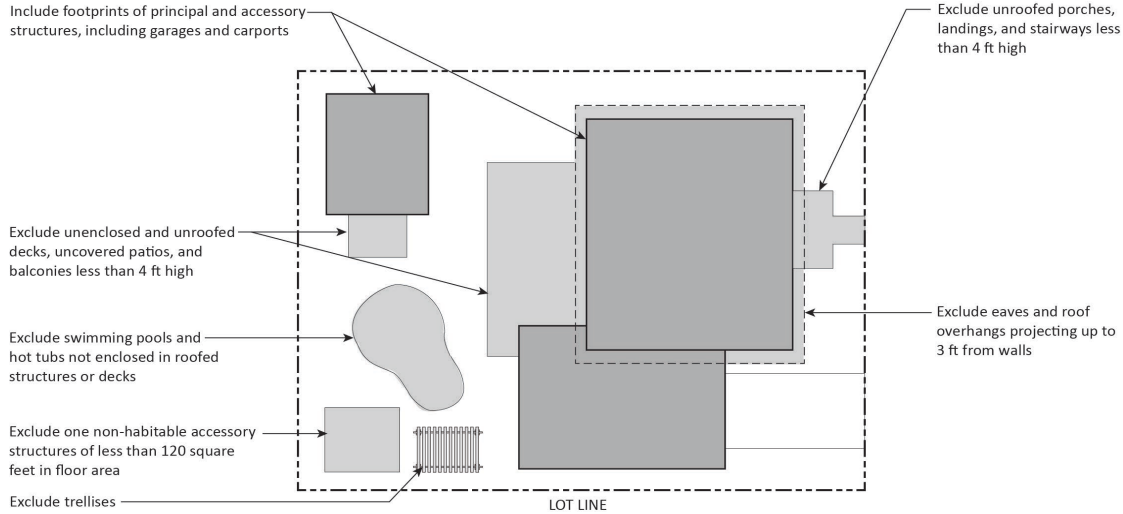
Figure 17.34.060: Determining Lot Coverage
