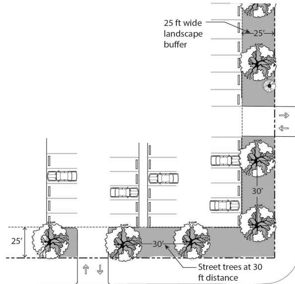
Figure 17.18.040.A, Landscape Buffer
