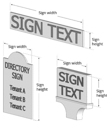
Figure 17.27.060.A: Signs on Background Panel
