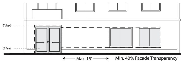
Figure 17.17.040.F: Building Transparency for SC District
