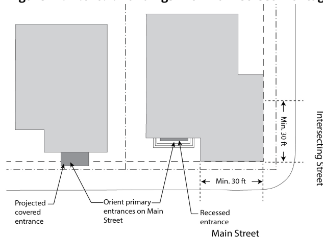
Figure 17.17.040.E: Buildings with Main Street Frontage
