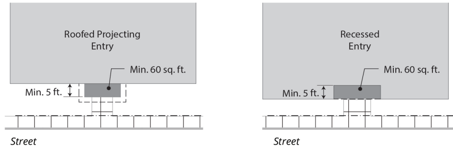
Figure 17.16.040.O: Entrances Serving Multiple Units
